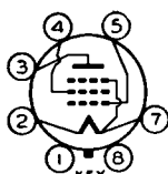
BOTTOM VIEW (G-6X)
